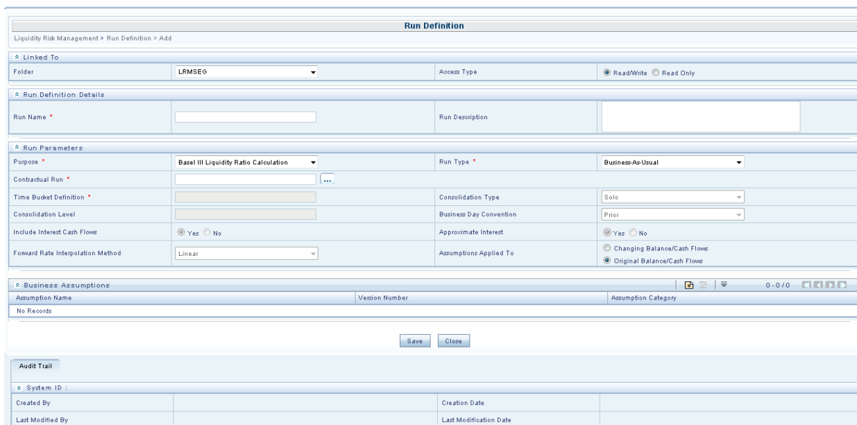
Figure 36 Run Definition - Contractual Business-As-Usual Run
